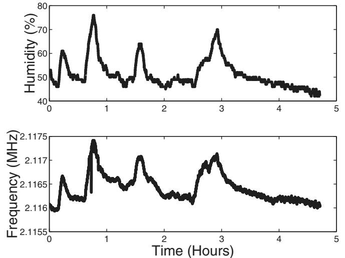
Fig. 15. Humidity measurement at 23°C.
