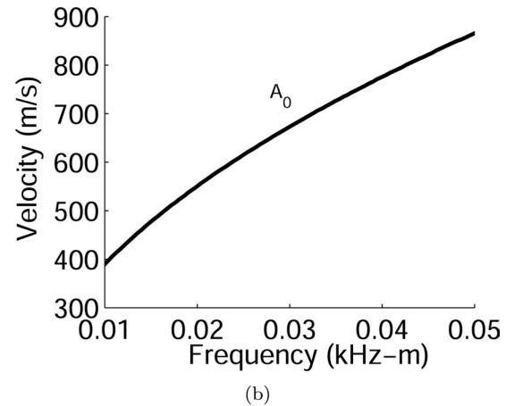
Fig. 1. (a) Select Lamb and Rayleigh velocities on silicon. (b) An expansion of the A_0 curve for frequency-thickness values near 0.038 kHz-m, the operating point of the devices discussed in this paper. The calculations used to create both plots treat silicon as an isotropic material. The constants are taken from [34] V_s = 5840.9 m/s, V_l = 8429.4 m/s.
