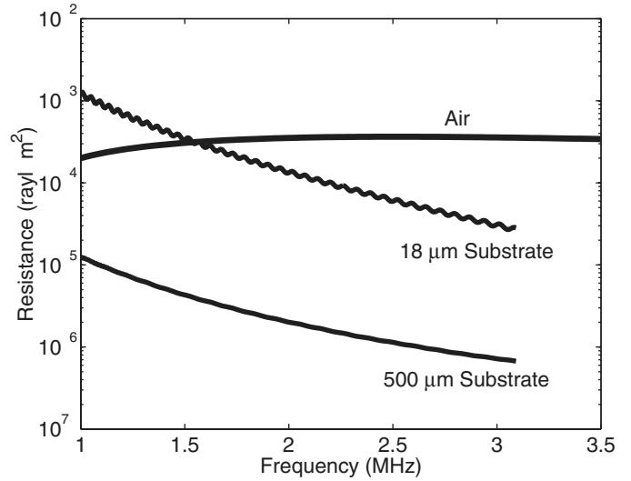
Fig. 9. Resistance presented to the membrane by the A_0 for an 18- \mu m substrate and a 500- \mu m substrate. The resistance of air as expressed in (9) is also shown as a point of reference. Constants for silicon are taken from (34): V_s = 5840.9 m/s, V_l = 8429.4 m/s, \rho = 2332 kg/m 3 . Constants for air are taken from [45]: \rho = 1.24 kg/m 3 , v = 344 m/s.
