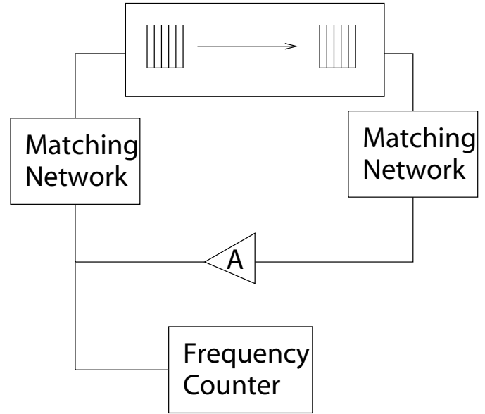
Fig. 3. Experimental setup of the delay-line oscillator.
