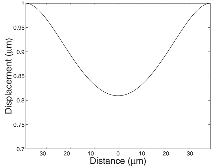
Fig. 6. Static membrane deflection as a function of location for a 77 \mu\text{m} wide membrane with a 1- \mu\text{m} gap. The ambient pressure on the membrane in this simulation is 101.3 kPa. The constants used in this simulation are Y_0 = 3.2 \times 10^{11} Pa, \sigma = 0.263 , \rho = 2843 kg/m 3 , T = 100 MPa.
