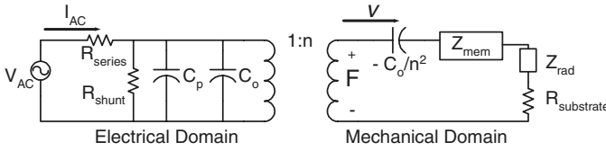
Fig. 4. Equivalent circuit model of a transmitting CMUT.
